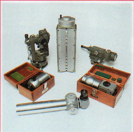
THEODOLITE, DUMPY LEVEL, TELESCOPE
