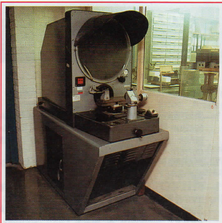
BATY R20C PROJECTOR
