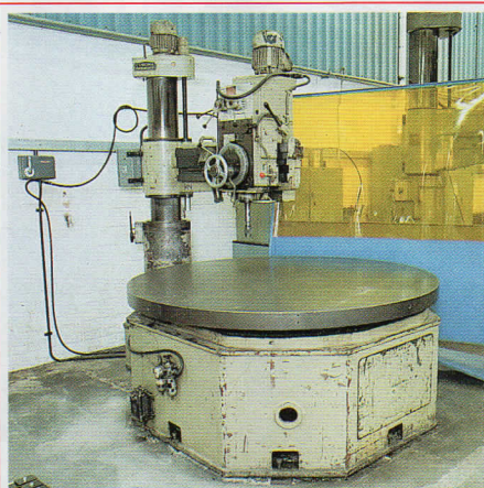
POLLARD 420 RADIAL DRILL & 72" TABLE
