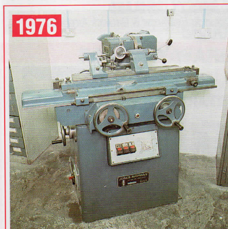
JONES & SHIPMAN 310T T & C GRINDER
