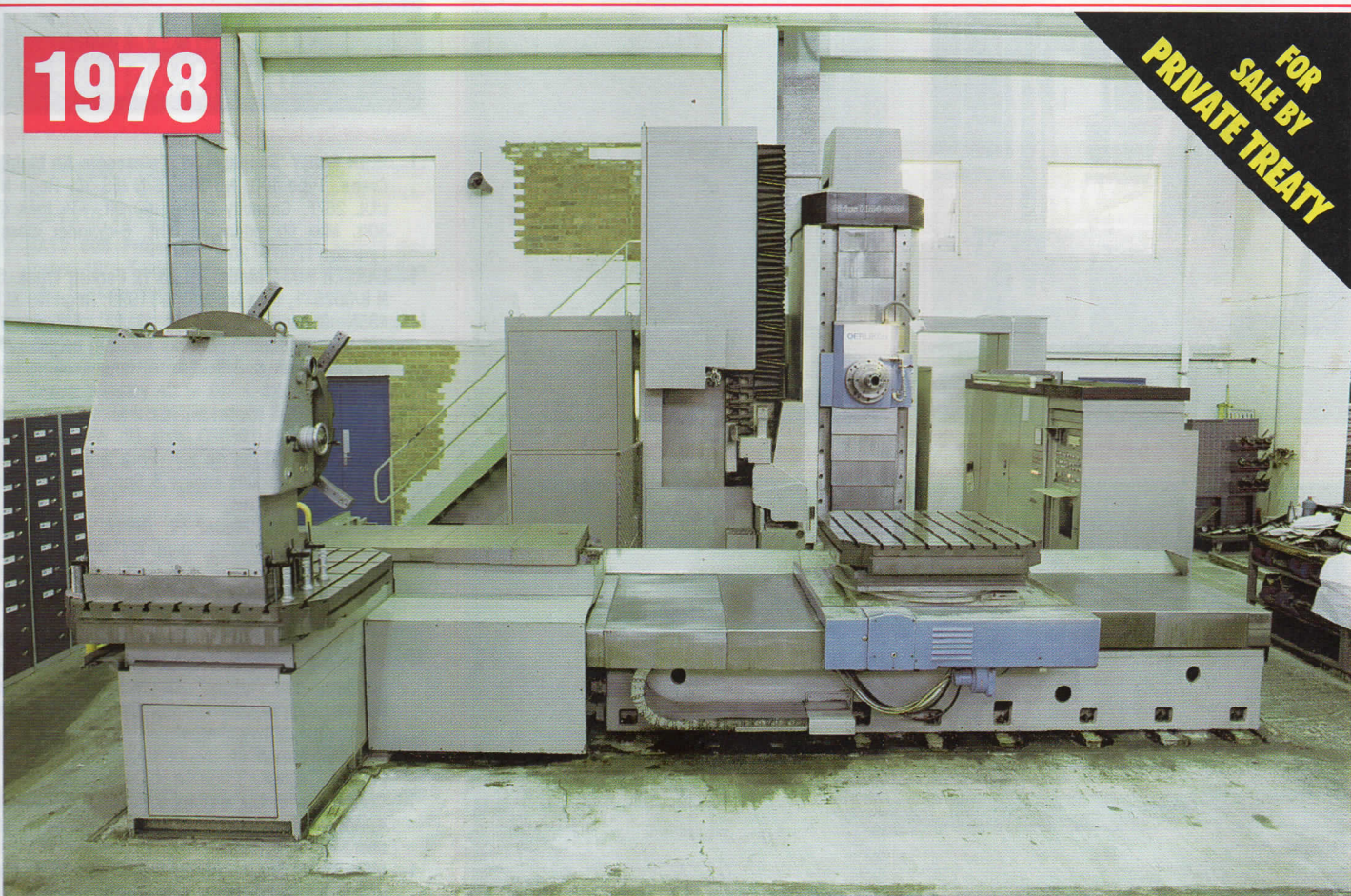
OERLIKON SIRIUS MODEL HM4-MCP 4-AXIS CNC HORIZONTAL MACHINING CENTRE
