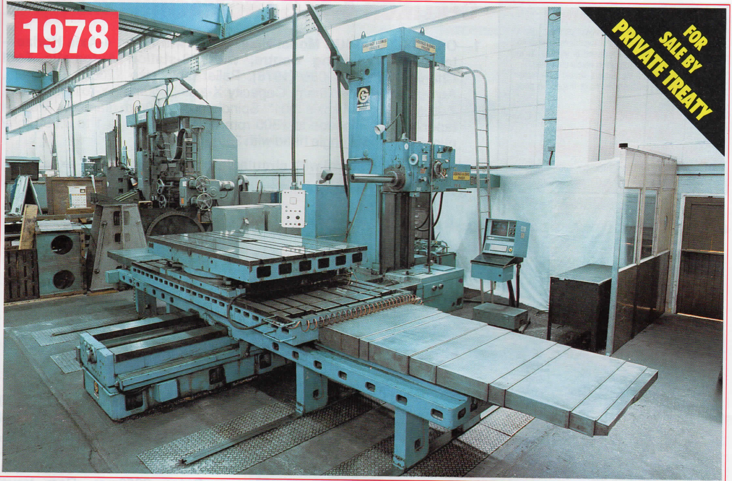
GIDDINGS & LEWIS-FRASER MODEL 80DP130 HORIZONTAL BORER
