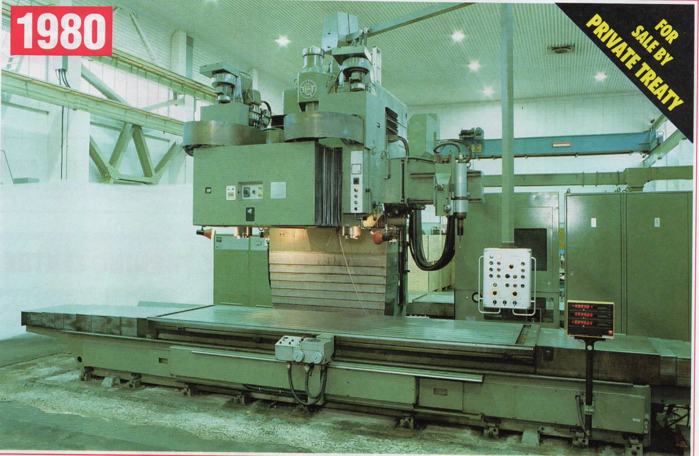
STARRAG LA RIGIDE MODEL KE275 TWIN SPINDLE VERTICAL COPY MILL
