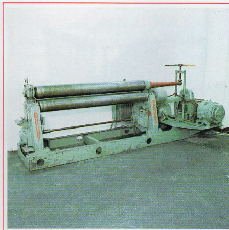
BRONX PBA36 INITIAL ROLLS
