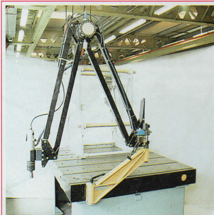
S & L MASKIN SINGLE HEAD TAPPER
